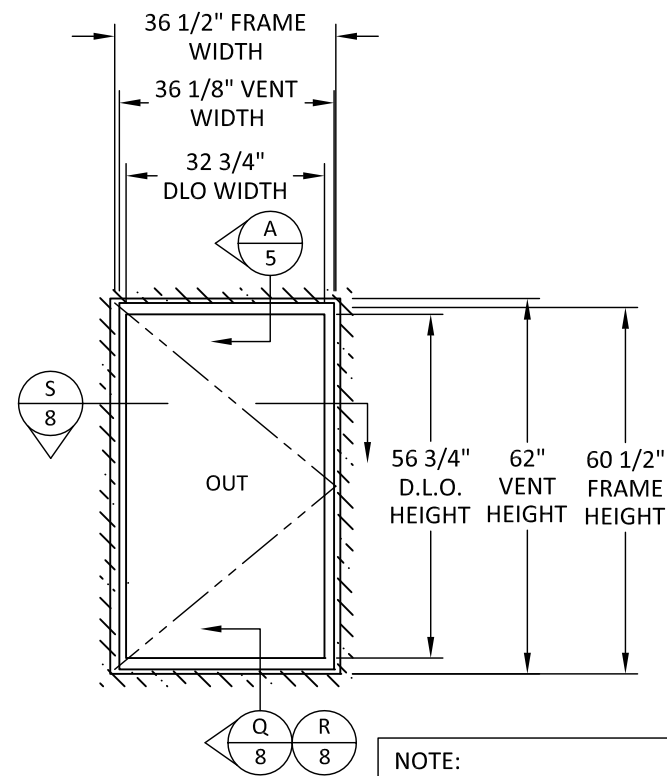
ELEVATION 2 OR 3 SIDED SSG CAPTURED HORIZONTALS
