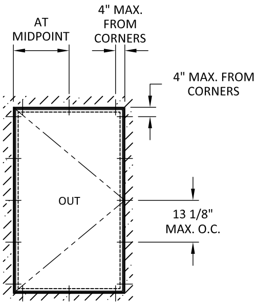
ANCHOR LAYOUT
