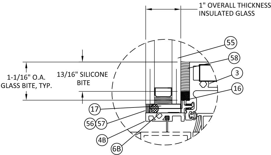
GLAZING DETAIL G2 CAPTURED VENT NON-IMPACT RATED
