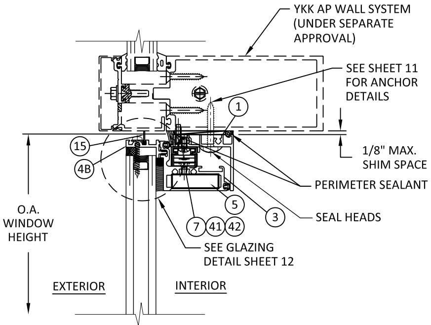
C 5 VERTICAL SECTION VENT HEAD - YKK AP WALL SYSTEM CAPTURED - FIELD GLAZED
