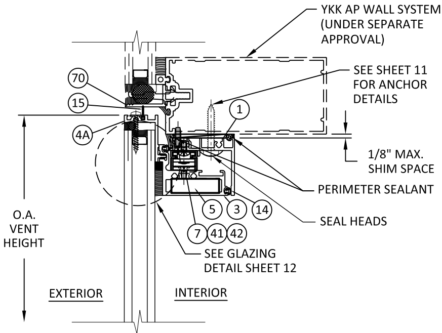
A 5 VERTICAL SECTION VENT HEAD - YKK AP WALL SYSTEM SSG - FIELD GLAZED
