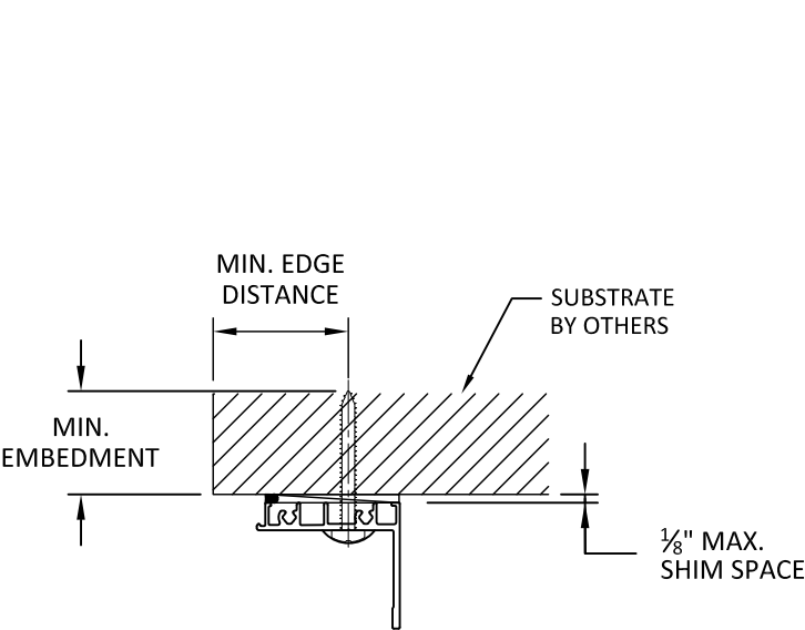
ANCHOR DETAIL
