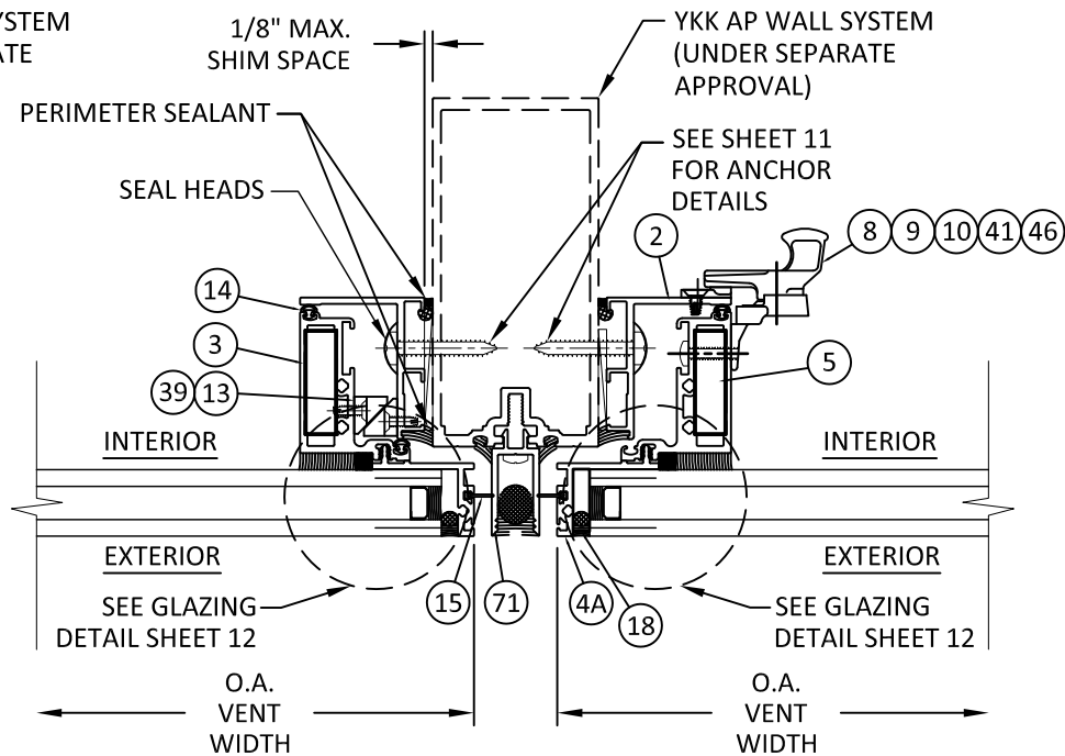
I 6 HORIZONTAL SECTION VENT HINGE & LOCK JAMBS - WALL SYSTEM SSG - FIELD GLAZED
