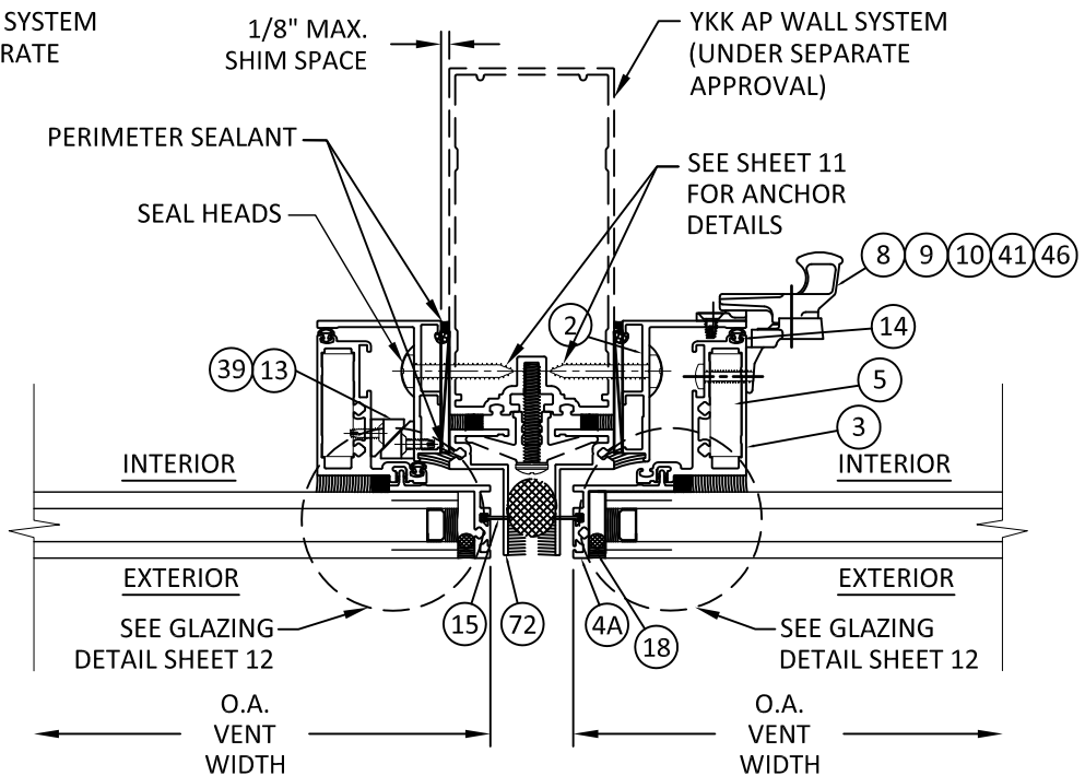
L 6 HORIZONTAL SECTION VENT HINGE & LOCK JAMBS - WALL SYSTEM SSG - SHOP GLAZED
