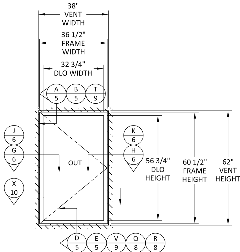
ELEVATION 4 SIDED SSG
