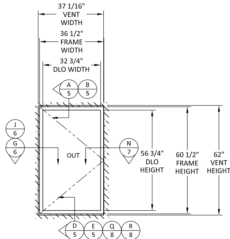
ELEVATION 3 SIDED SSG CAPTURED VERTICAL
